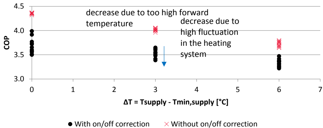
Figure 32. Results from simulation of the efficiency of a heat pump dependent on the forward temperature and fluctuation of the flow rate through the heating system (Jensen, Olesen and Paulsen, 2014).
