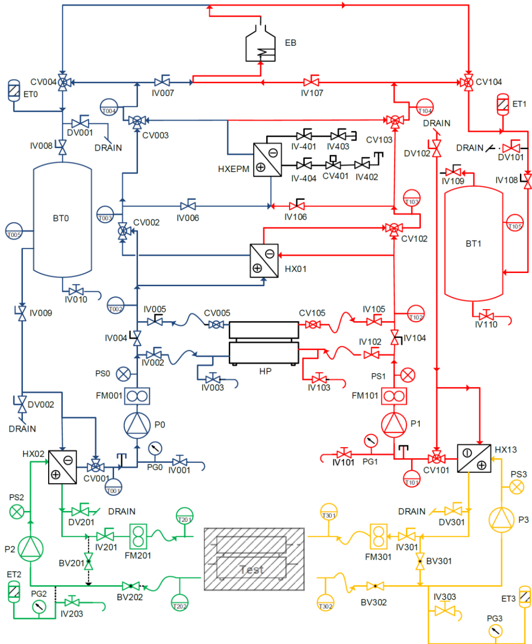
Figure 36. Hydronic loops of the Semi-Virtual Laboratory.
